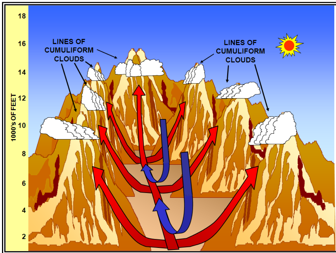
Figure 10-19. Valley Breeze
