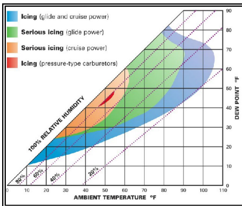
Figure 20-3. Carburetor Icing
