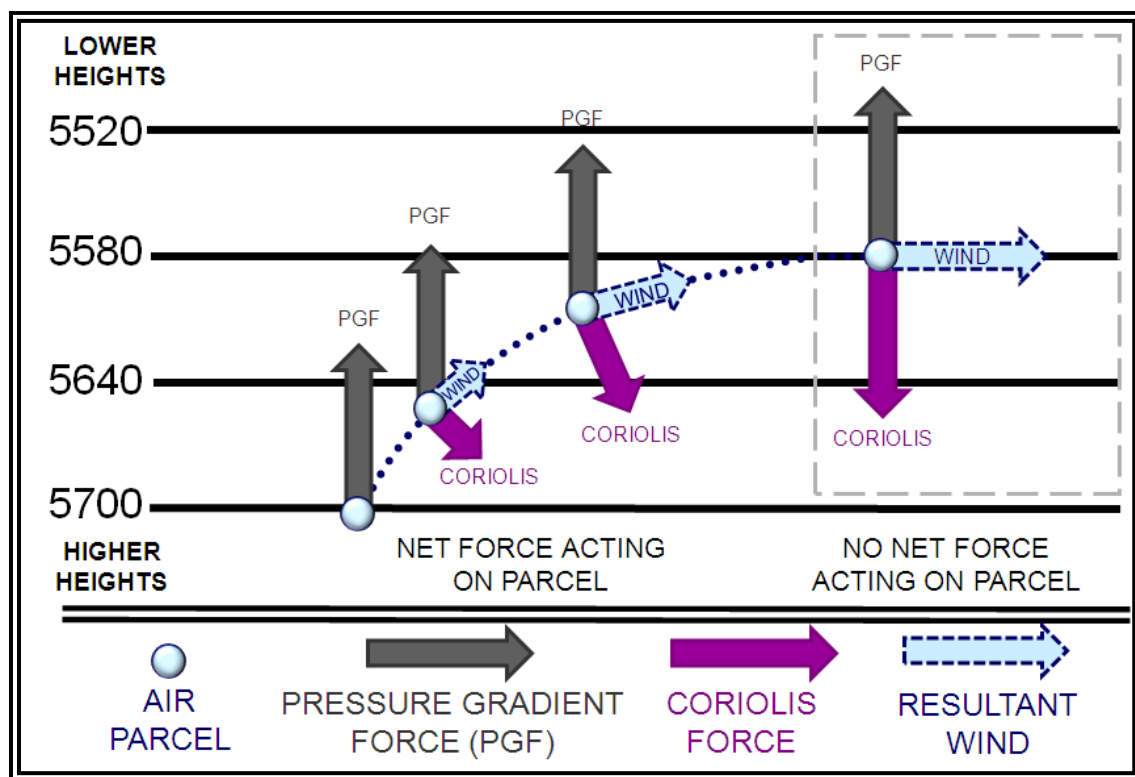
Figure 10-8. Geostrophic Wind
