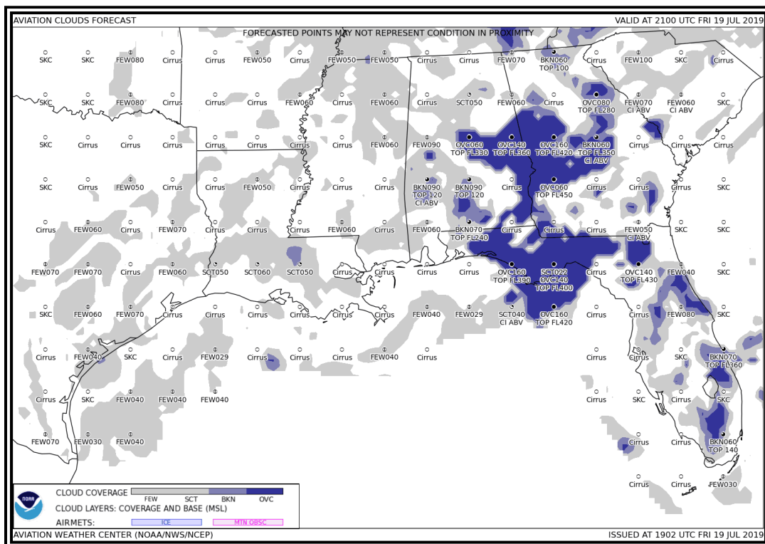
Figure 27-4. Aviation Clouds Forecast Example
