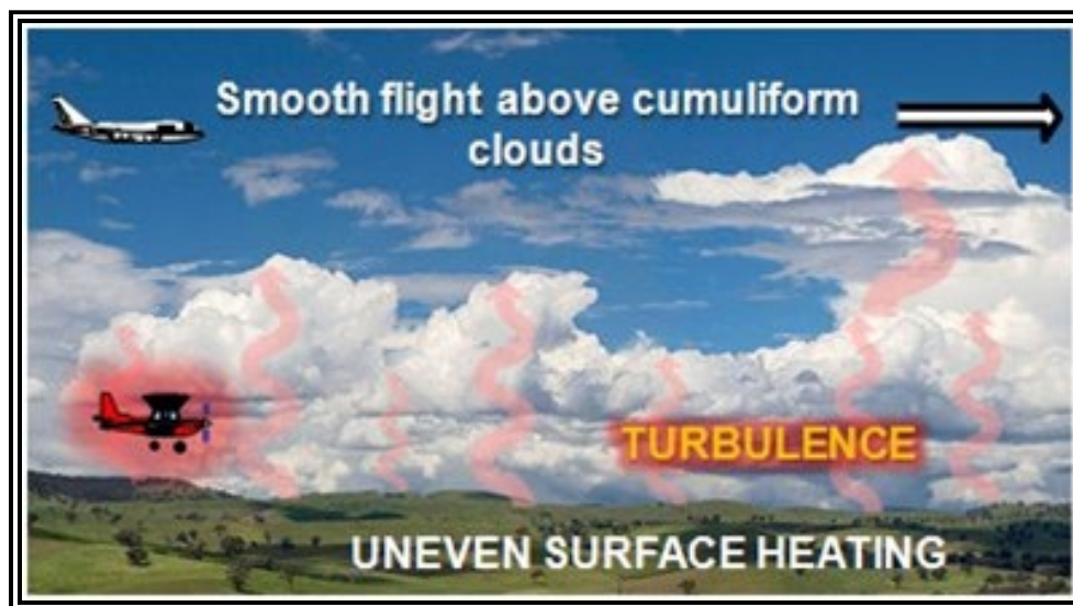
Figure 19-1. Convective Turbulence
